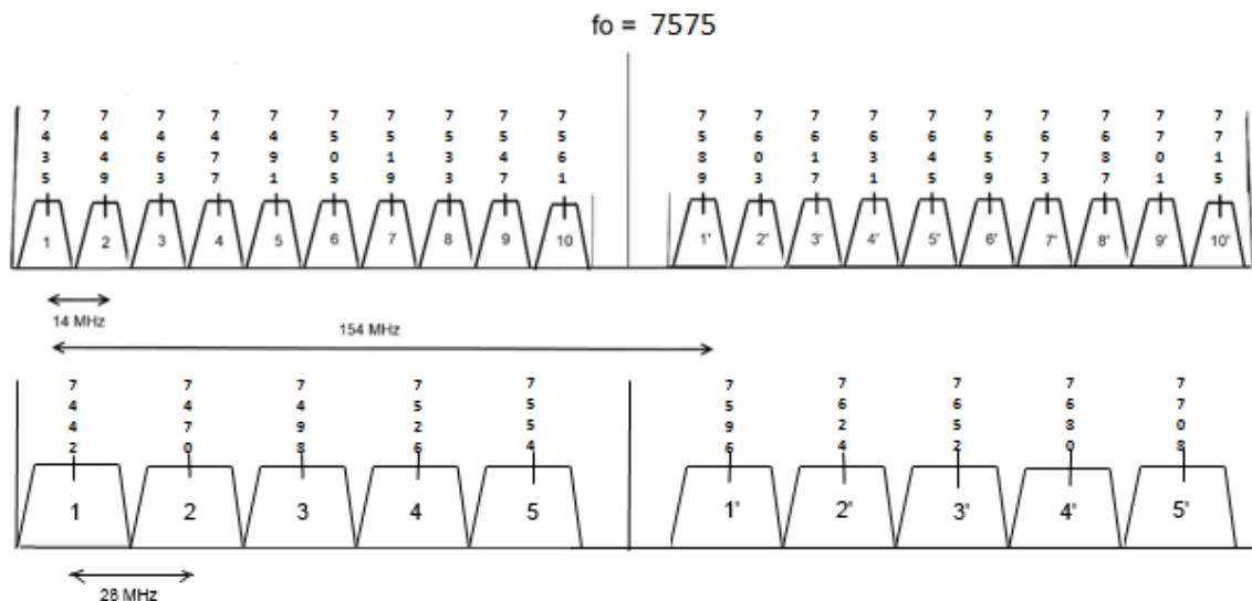
Alternative Arrangements with 154 MHz Duplex.
